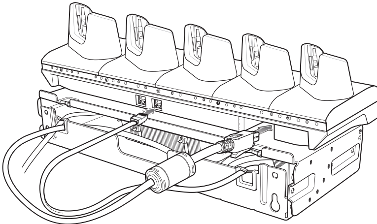
Figure 2-32 Connect Cables
