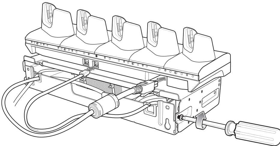
Figure 2-33 Secure Top and Bottom Tray
