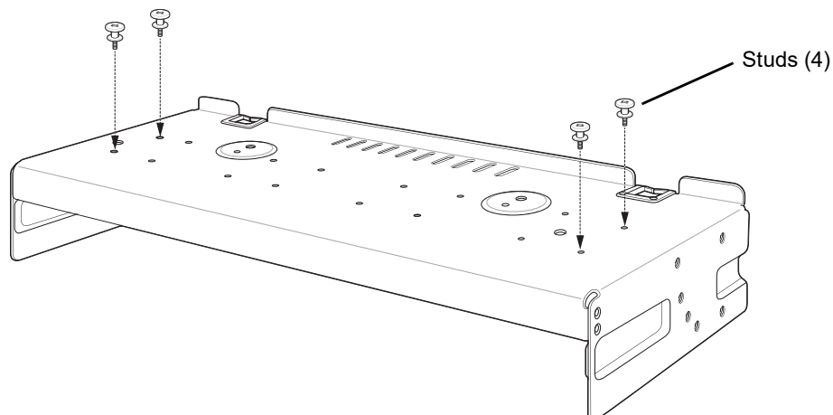
Figure 2-28 Install Studs
