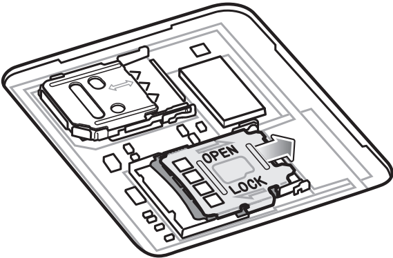
Figure 1-4 Lift the SIM Card Holder
