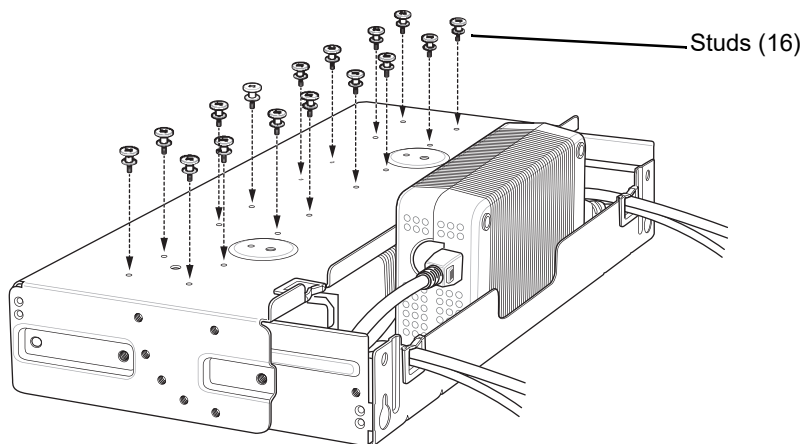
Figure 2-36 Install Studs
