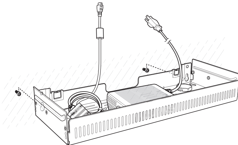
Figure 2-45 Horizontal Installation
